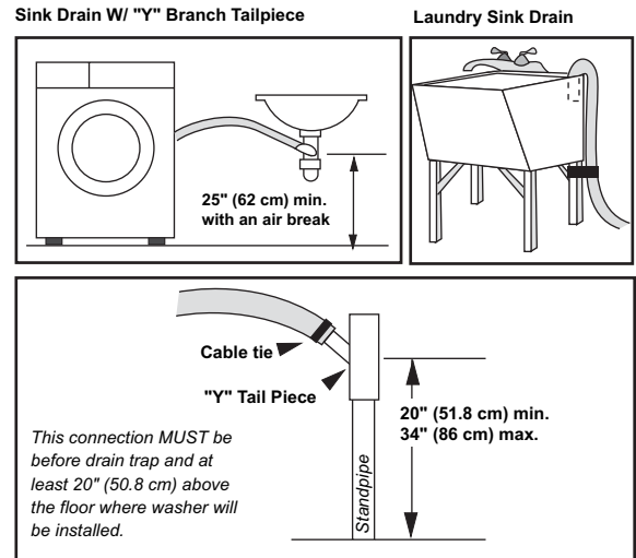
Floor Standpipe w/ "Y" Branch Tail Piece
