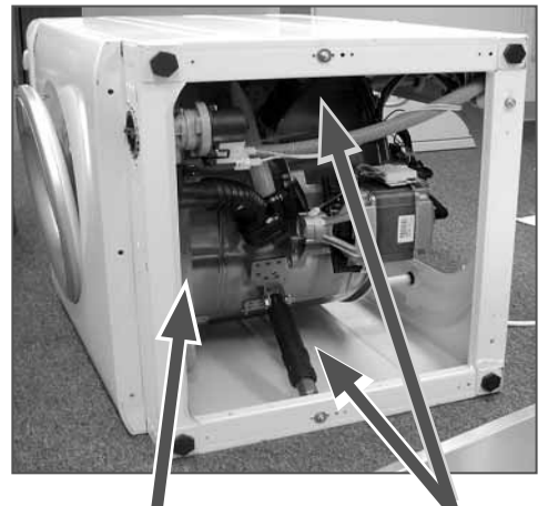
Bottom/Front Counter Weight
